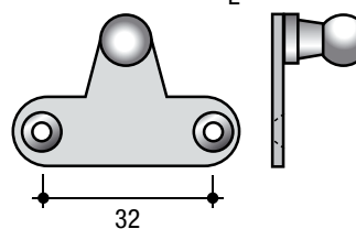
Attacco per ante in alluminio Attachment for aluminium frames Attaque cadres Aluminium
