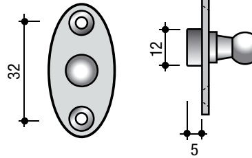
Attacco per fianco Attachment for side panel Attaque cadres
