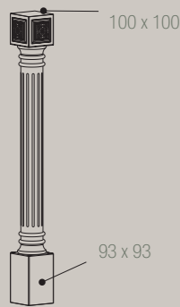
GAMBA ISOLA C/DECORO LEG FOR PENINSULA "H" = 870
