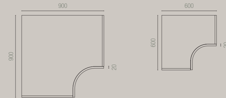
BASE CONCAVA CURVA 900 x 900 E PENSILE CONCAVO CURVO 600 x 600 INTERNAL CURVED BASE AND WALL UNITS
