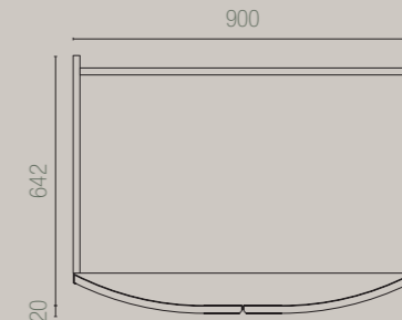
COPPIA ANTE CURVE CURVED DOOR (PAIR)
