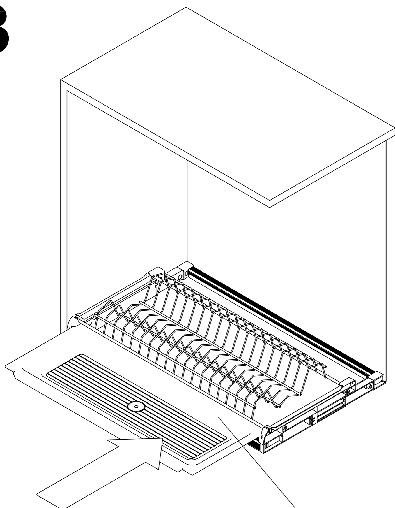
Gocciolatoio / Drip Tray 602
