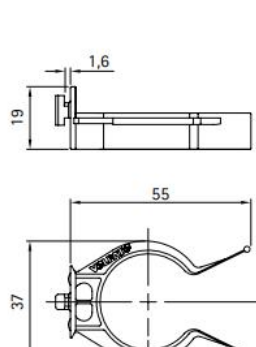
Per zoccoli in plastica e alluminio For plastic and aluminium plinths
