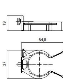
Sistema Gancio Easyfit Easyfit clip system Per zoccoli in plastica e alluminio For plastic and aluminium plinths
